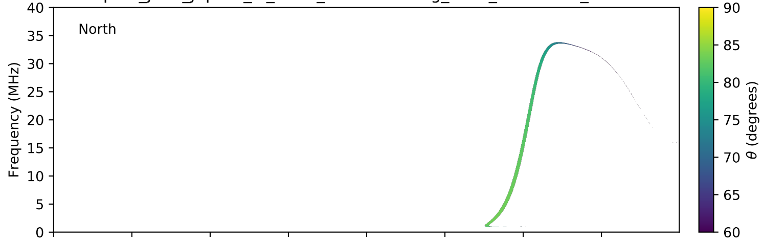
expres_juno_jupiter_io_isaac_lossc-wid1deg_3kev_20181025_v01.cdf
