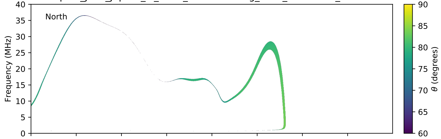
expres_juno_jupiter_io_isaac_lossc-wid1deg_3kev_20181024_v01.cdf
