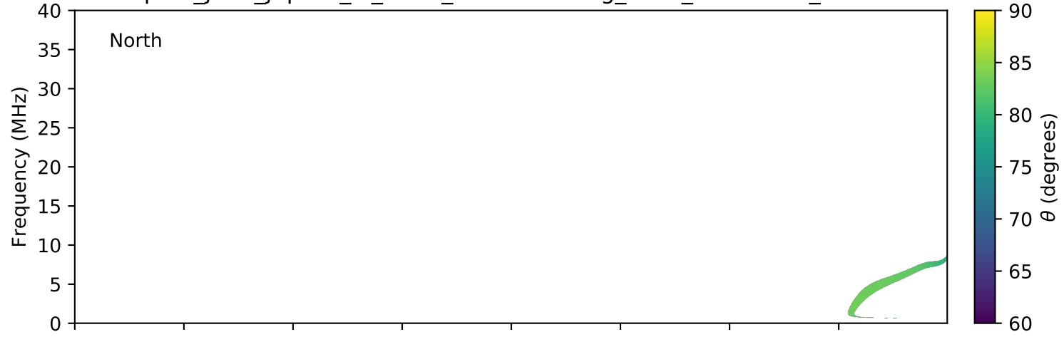
expres_juno_jupiter_io_isaac_lossc-wid1deg_3kev_20181023_v01.cdf
