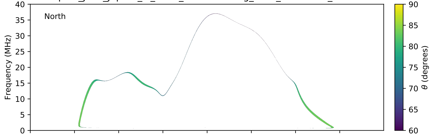
expres_juno_jupiter_io_isaac_lossc-wid1deg_3kev_20181022_v01.cdf
