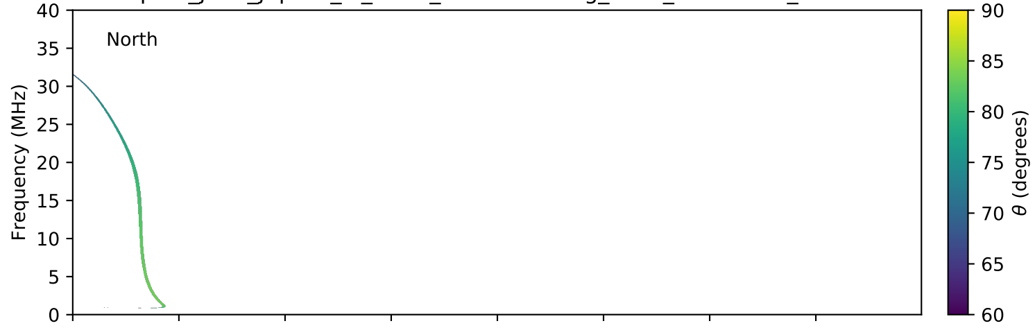
expres_juno_jupiter_io_isaac_lossc-wid1deg_3kev_20181021_v01.cdf
