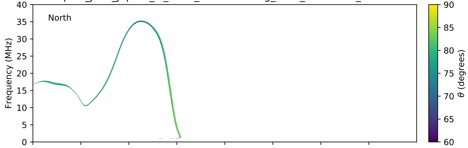
expres_juno_jupiter_io_isaac_lossc-wid1deg_3kev_20181019_v01.cdf
