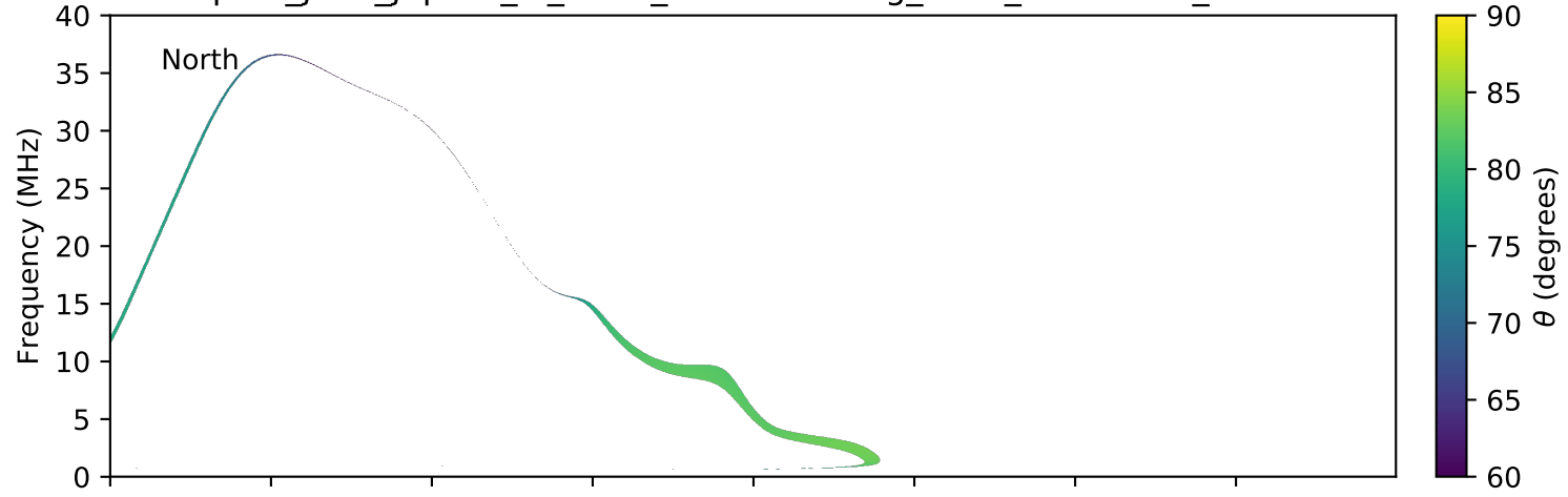
expres_juno_jupiter_io_isaac_lossc-wid1deg_3kev_20181017_v01.cdf
