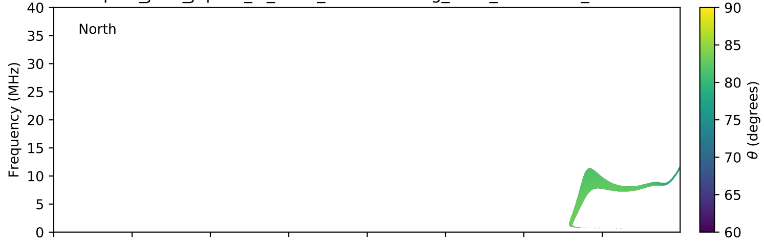
expres_juno_jupiter_io_isaac_lossc-wid1deg_3kev_20181016_v01.cdf
