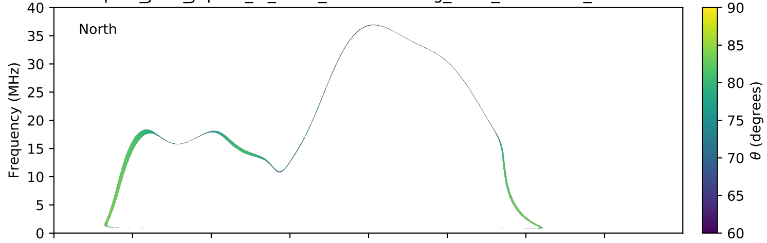
expres_juno_jupiter_io_isaac_lossc-wid1deg_3kev_20181015_v01.cdf
