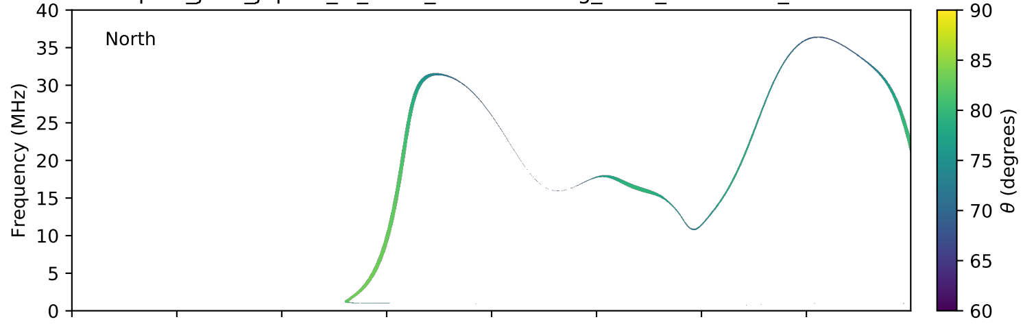
expres_juno_jupiter_io_isaac_lossc-wid1deg_3kev_20181013_v01.cdf
