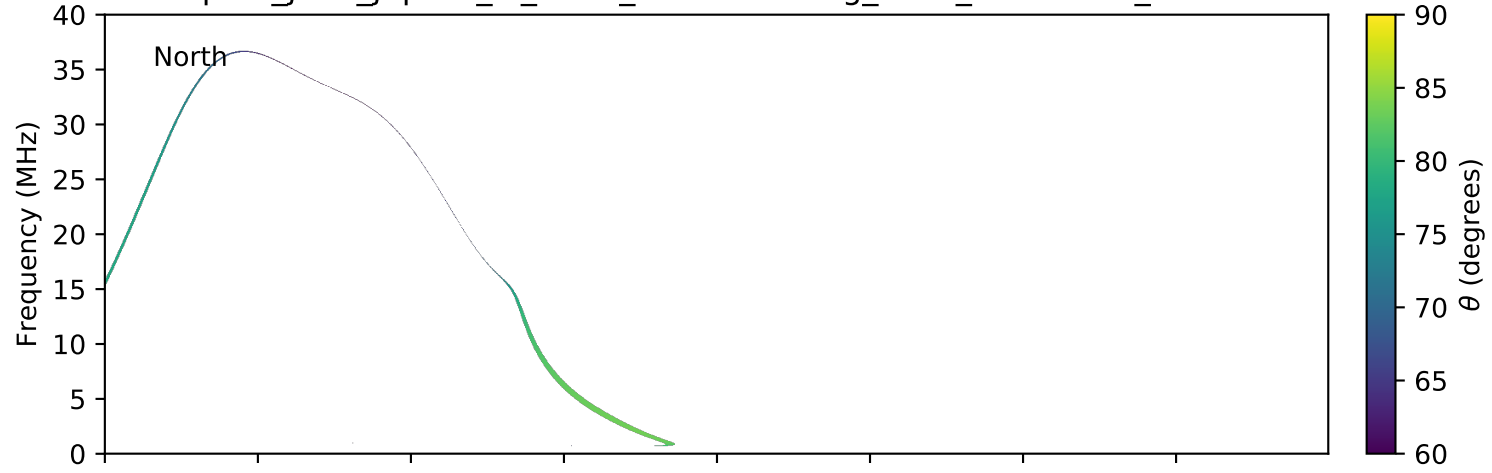
expres_juno_jupiter_io_isaac_lossc-wid1deg_3kev_20181010_v01.cdf
