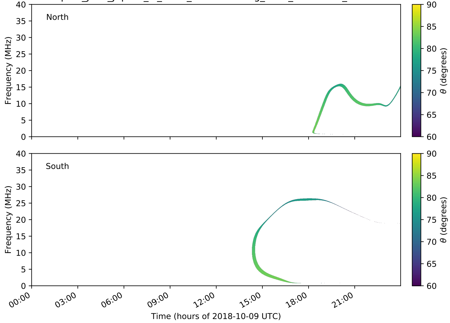
expres_juno_jupiter_io_isaac_lossc-wid1deg_3kev_20181009_v01.cdf
