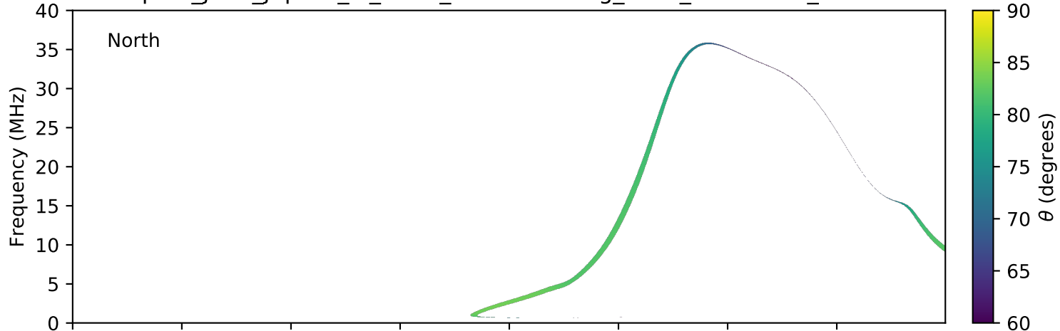
expres_juno_jupiter_io_isaac_lossc-wid1deg_3kev_20181004_v01.cdf
