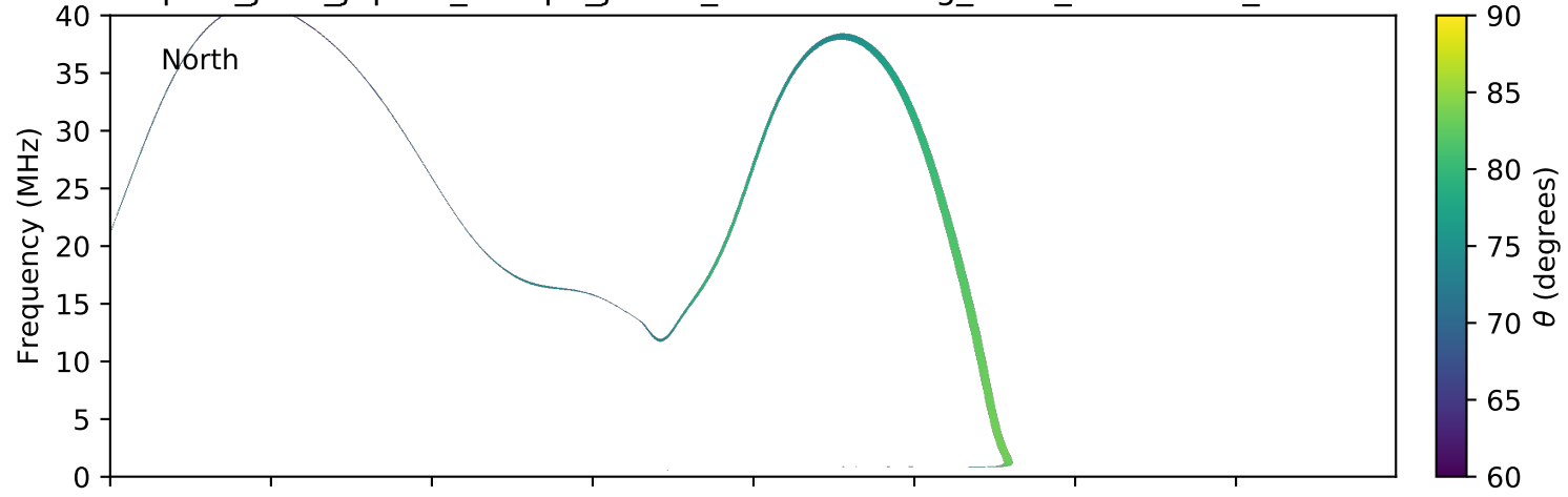
expres_juno_jupiter_europa_jrm09_lossc-wid1deg_3kev_20181027_v01.cdf
