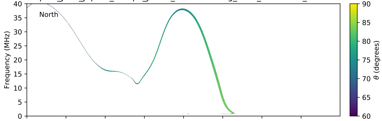
expres_juno_jupiter_europa_jrm09_lossc-wid1deg_3kev_20181025_v01.cdf
