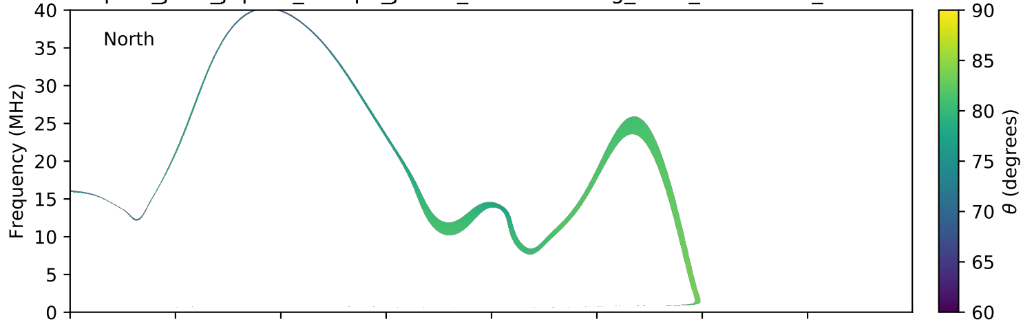
expres_juno_jupiter_europa_jrm09_lossc-wid1deg_3kev_20181024_v01.cdf
