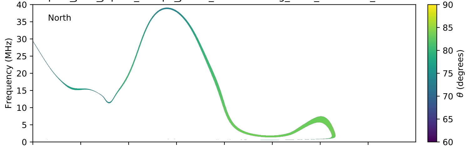
expres_juno_jupiter_europa_jrm09_lossc-wid1deg_3kev_20181021_v01.cdf
