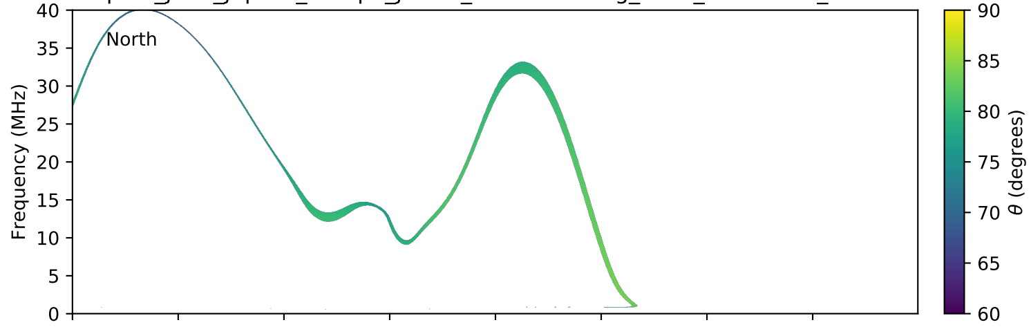
expres_juno_jupiter_europa_jrm09_lossc-wid1deg_3kev_20181020_v01.cdf
