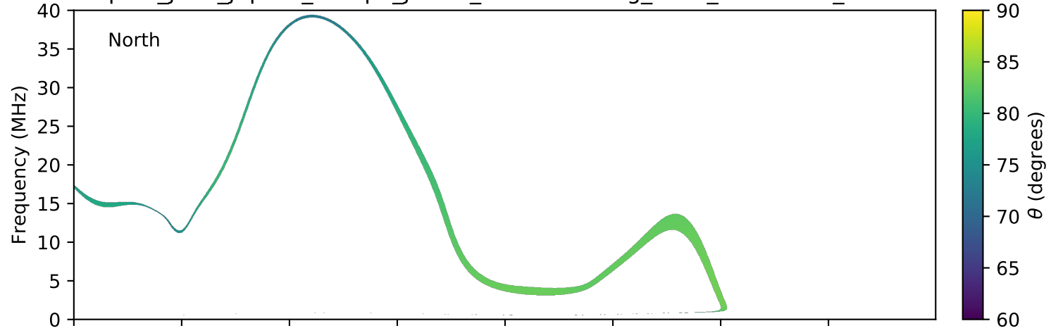
expres_juno_jupiter_europa_jrm09_lossc-wid1deg_3kev_20181019_v01.cdf
