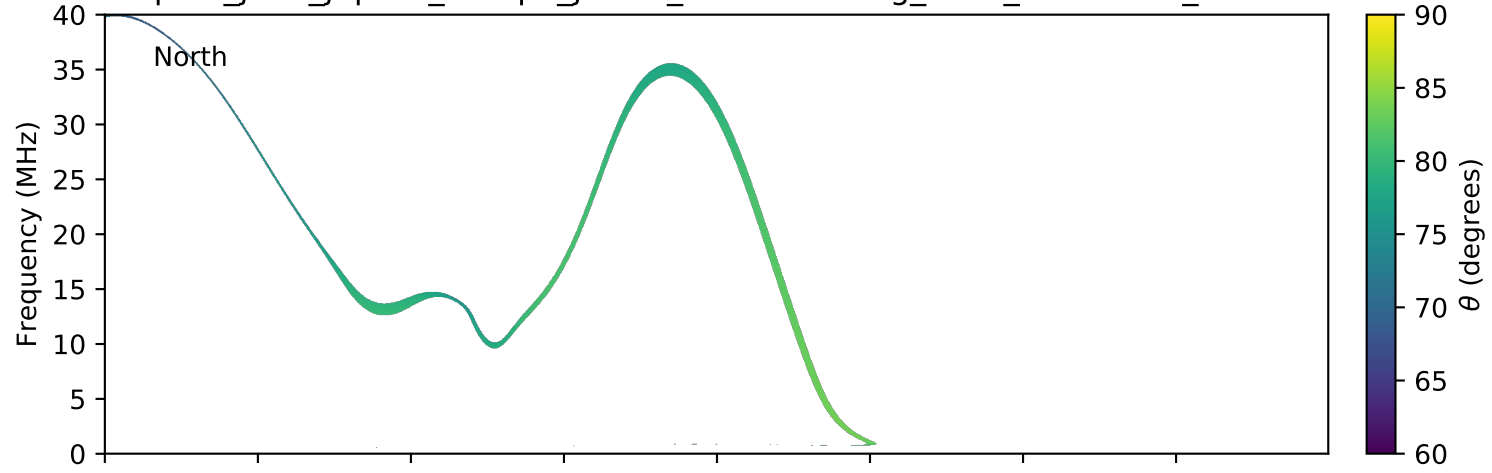
expres_juno_jupiter_europa_jrm09_lossc-wid1deg_3kev_20181018_v01.cdf
