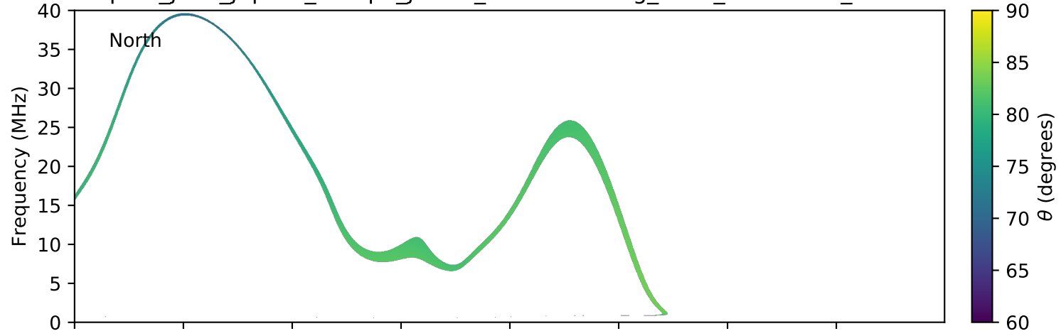
expres_juno_jupiter_europa_jrm09_lossc-wid1deg_3kev_20181015_v01.cdf
