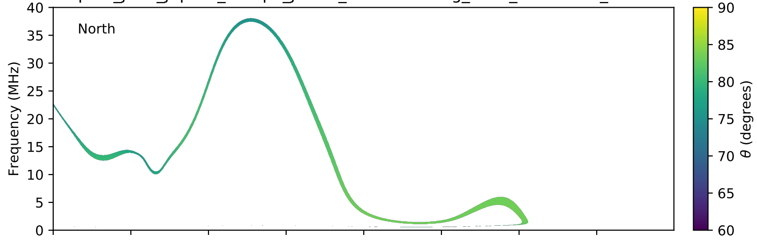
expres_juno_jupiter_europa_jrm09_lossc-wid1deg_3kev_20181014_v01.cdf
