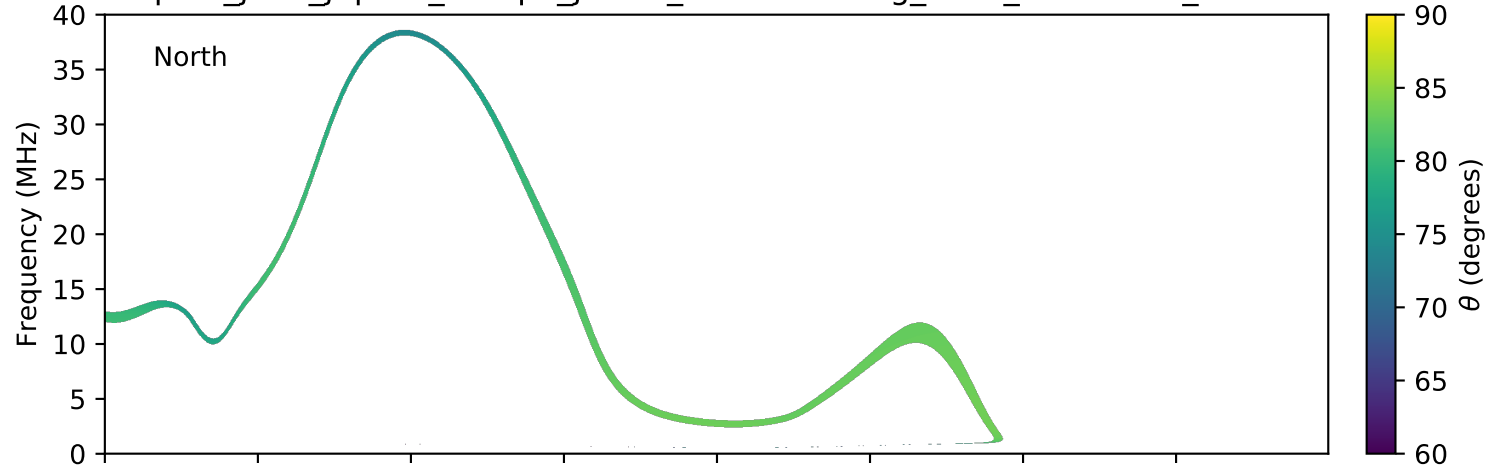
expres_juno_jupiter_europa_jrm09_lossc-wid1deg_3kev_20181012_v01.cdf
