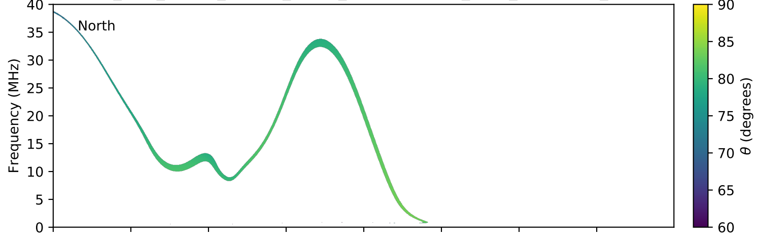
expres_juno_jupiter_europa_jrm09_lossc-wid1deg_3kev_20181011_v01.cdf
