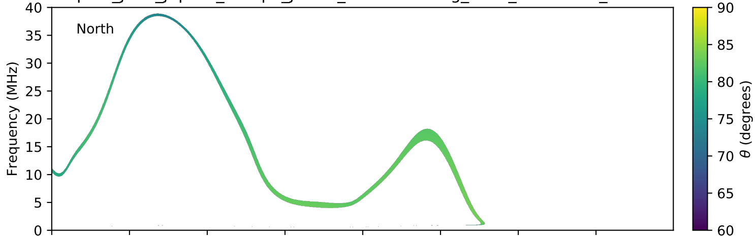
expres_juno_jupiter_europa_jrm09_lossc-wid1deg_3kev_20181010_v01.cdf
