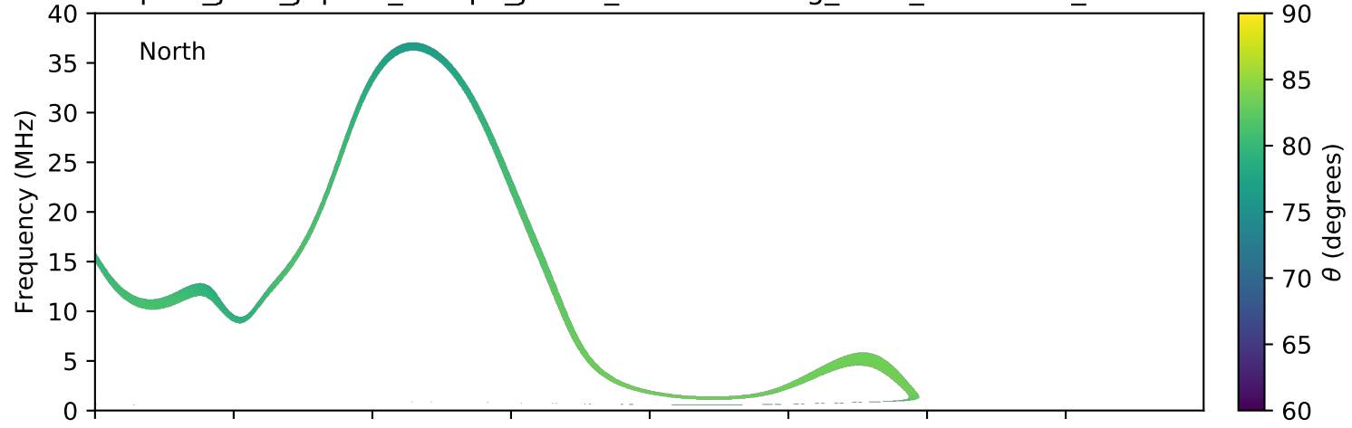
expres_juno_jupiter_europa_jrm09_lossc-wid1deg_3kev_20181007_v01.cdf
