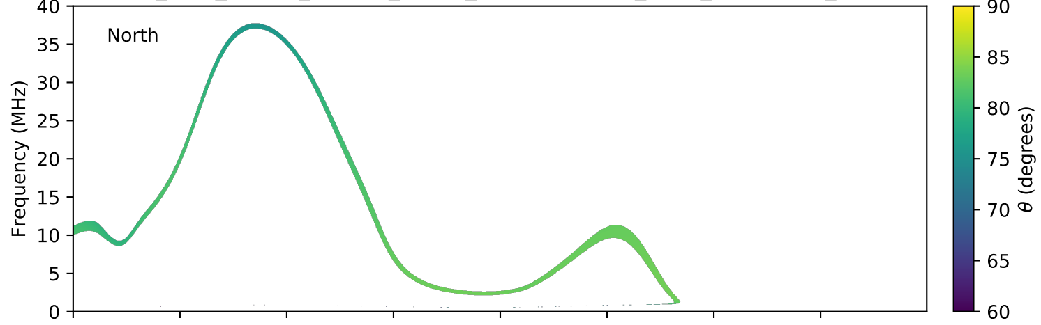
expres_juno_jupiter_europa_jrm09_lossc-wid1deg_3kev_20181005_v01.cdf
