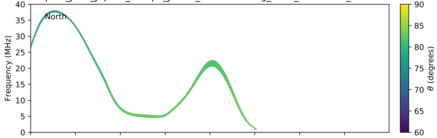
expres_juno_jupiter_europa_jrm09_lossc-wid1deg_3kev_20181001_v01.cdf
