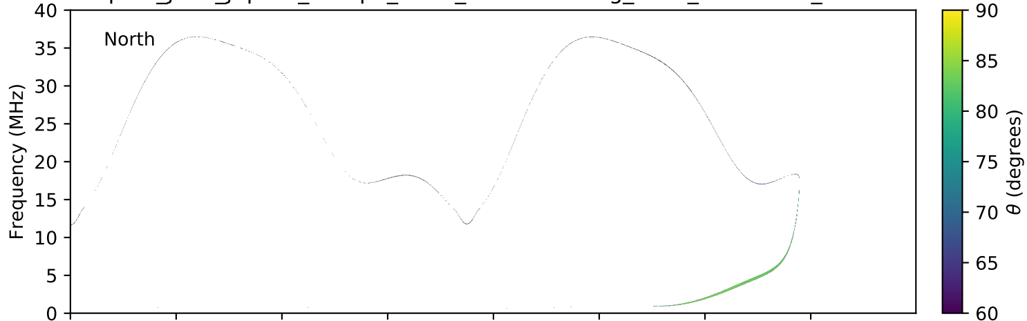
expres_juno_jupiter_europa_isaac_lossc-wid1deg_3kev_20181029_v01.cdf
