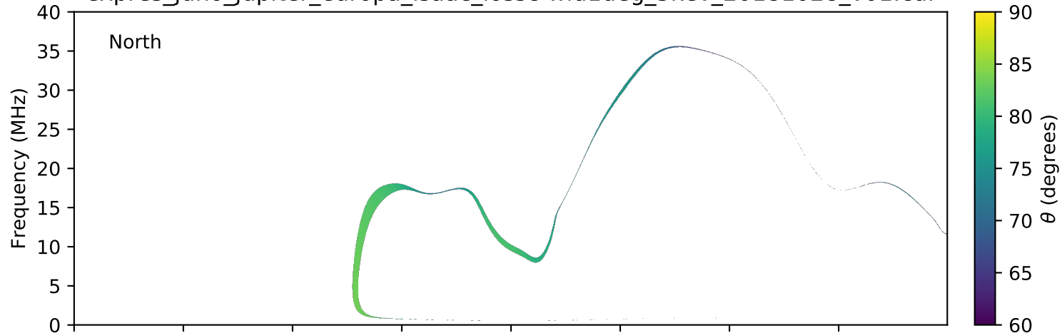
expres_juno_jupiter_europa_isaac_lossc-wid1deg_3kev_20181028_v01.cdf
