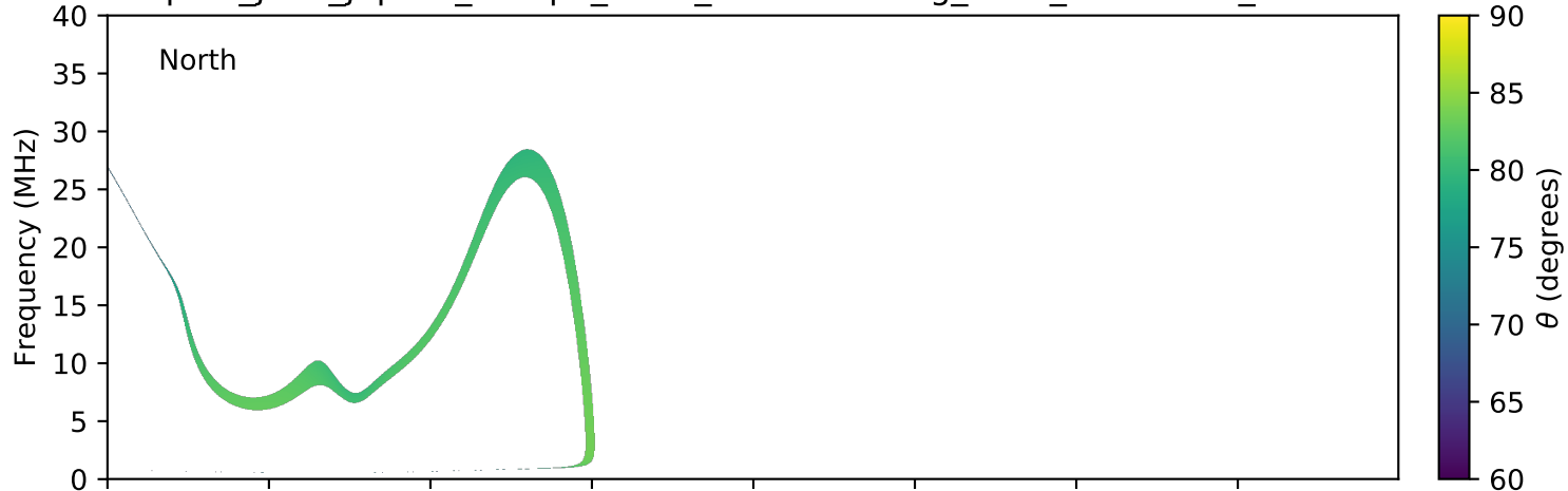
expres_juno_jupiter_europa_isaac_lossc-wid1deg_3kev_20181026_v01.cdf
