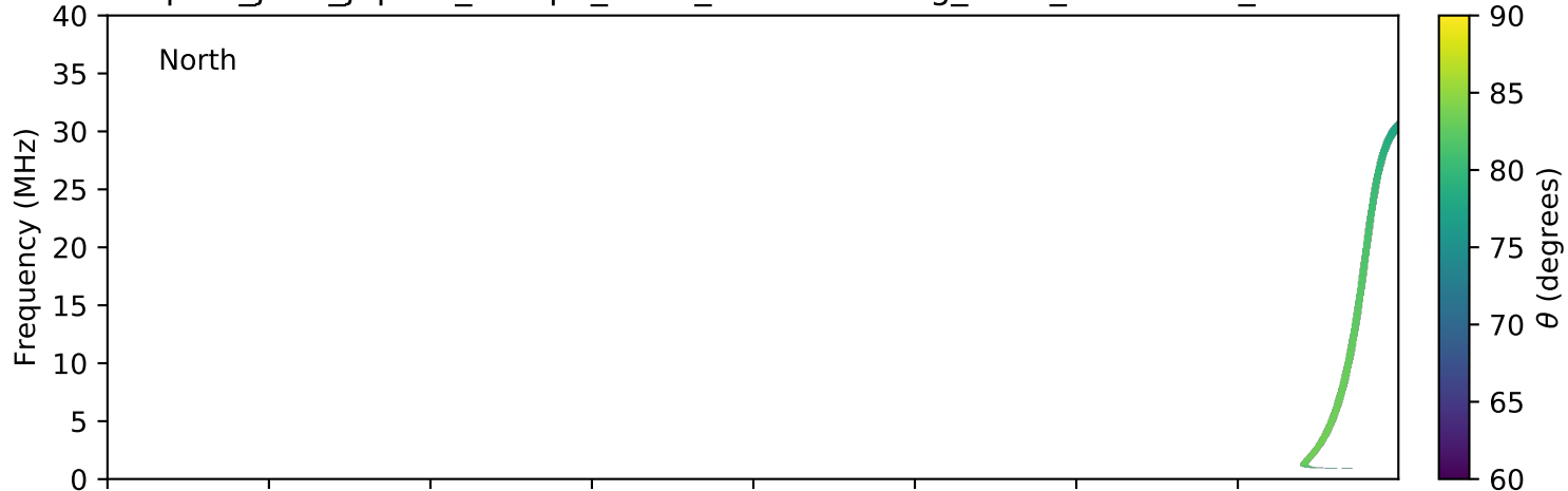
expres_juno_jupiter_europa_isaac_lossc-wid1deg_3kev_20181024_v01.cdf
