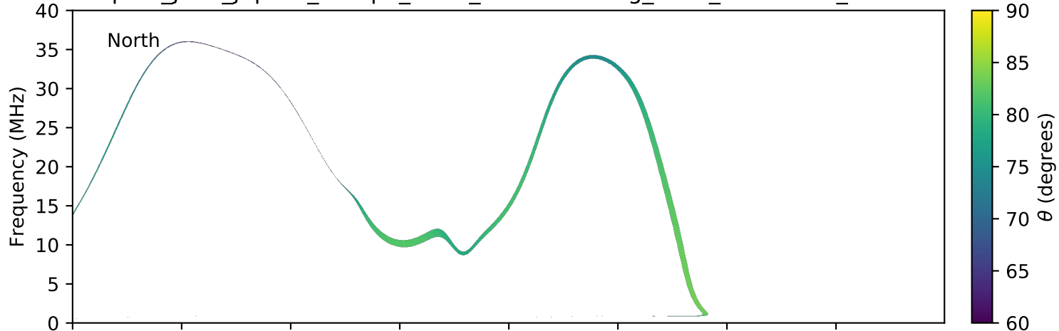
expres_juno_jupiter_europa_isaac_lossc-wid1deg_3kev_20181022_v01.cdf
