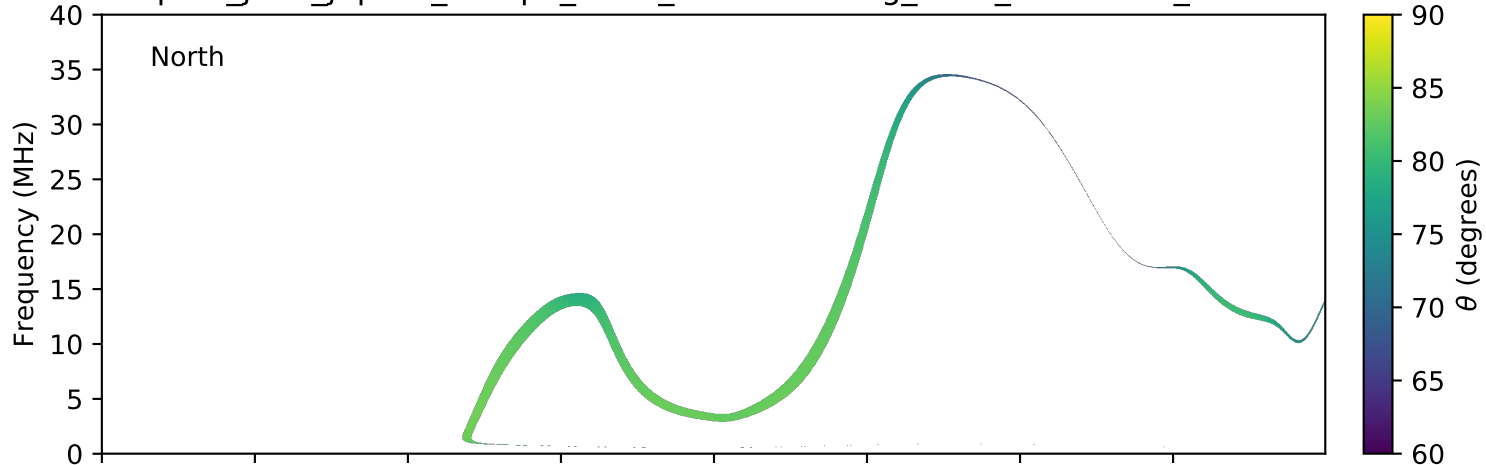
expres_juno_jupiter_europa_isaac_lossc-wid1deg_3kev_20181021_v01.cdf
