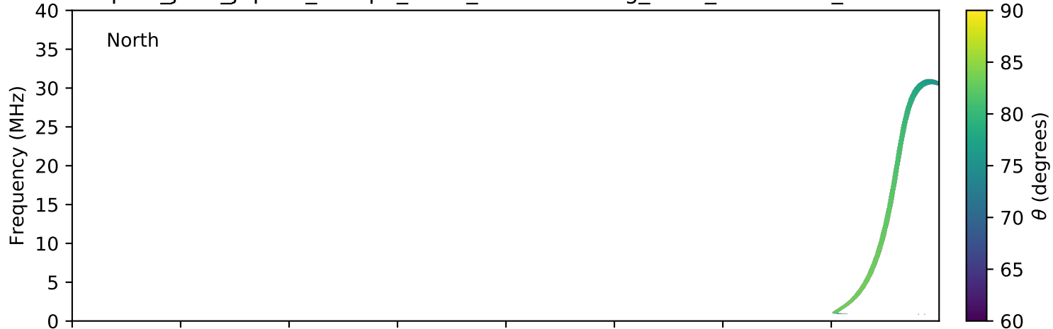
expres_juno_jupiter_europa_isaac_lossc-wid1deg_3kev_20181017_v01.cdf
