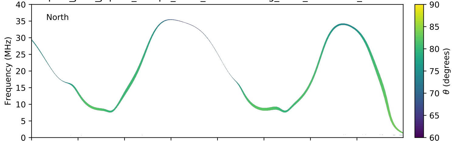
expres_juno_jupiter_europa_isaac_lossc-wid1deg_3kev_20181011_v01.cdf
