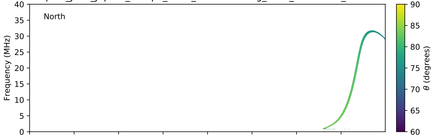
expres_juno_jupiter_europa_isaac_lossc-wid1deg_3kev_20181010_v01.cdf
