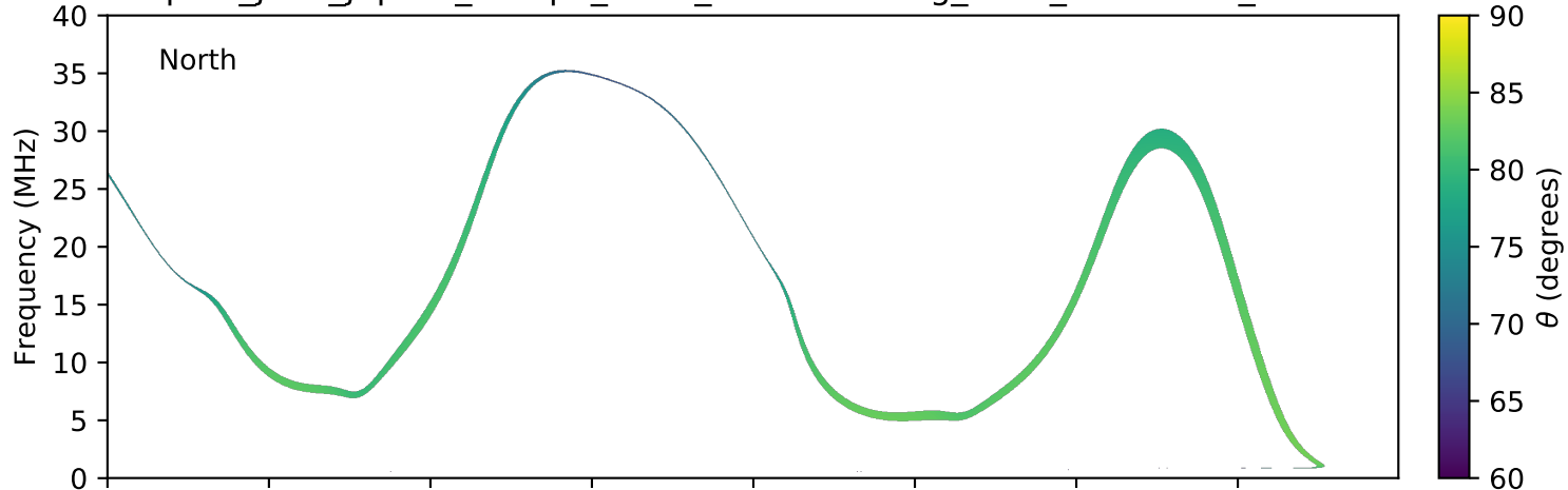
expres_juno_jupiter_europa_isaac_lossc-wid1deg_3kev_20181004_v01.cdf
