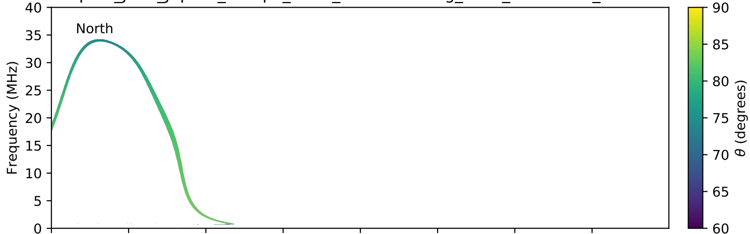
expres_juno_jupiter_europa_isaac_lossc-wid1deg_3kev_20181001_v01.cdf
