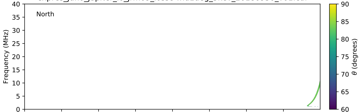
expres_juno_jupiter_io_jrm09_lossc-wid1deg_3kev_20180930_v01.cdf
