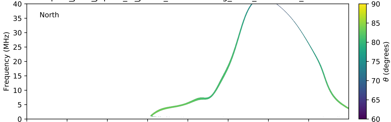
expres_juno_jupiter_io_jrm09_lossc-wid1deg_3kev_20180927_v01.cdf
