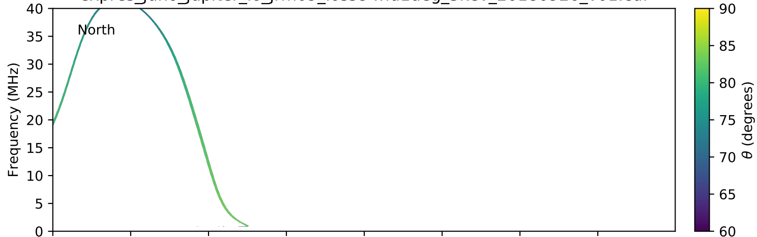
expres_juno_jupiter_io_jrm09_lossc-wid1deg_3kev_20180926_v01.cdf
