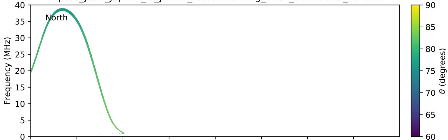
expres_juno_jupiter_io_jrm09_lossc-wid1deg_3kev_20180919_v01.cdf
