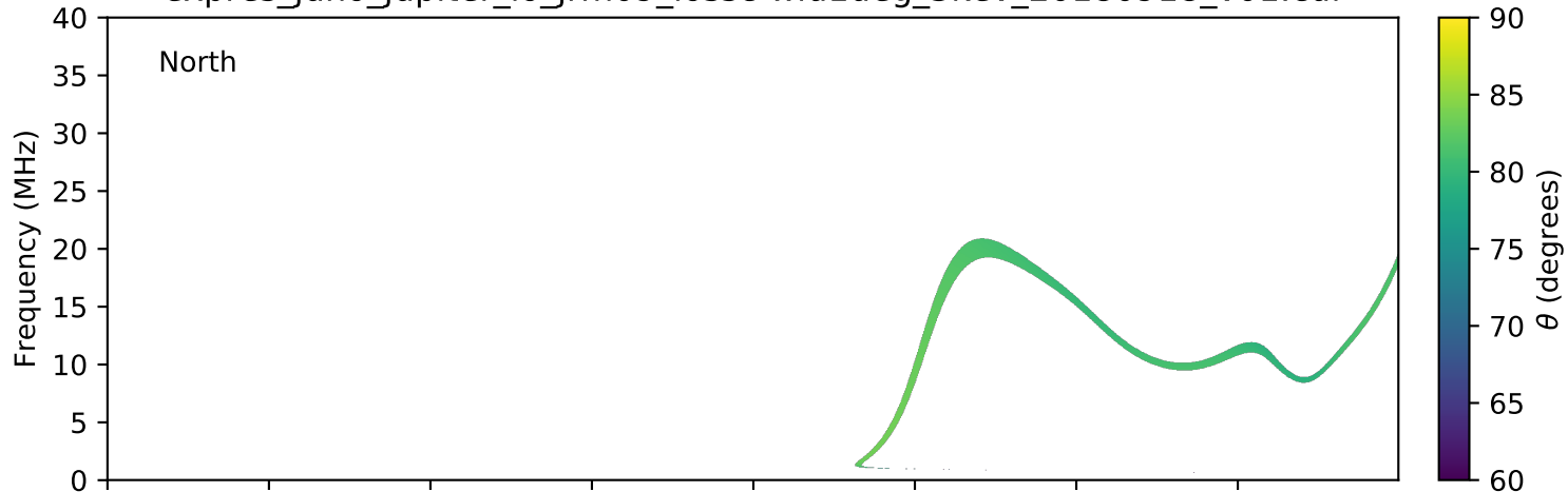
expres_juno_jupiter_io_jrm09_lossc-wid1deg_3kev_20180918_v01.cdf
