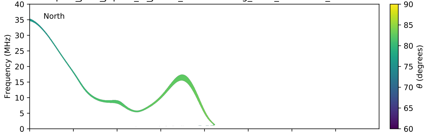
expres_juno_jupiter_io_jrm09_lossc-wid1deg_3kev_20180917_v01.cdf
