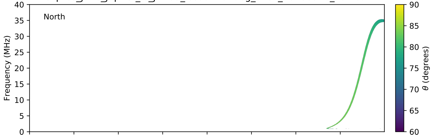
expres_juno_jupiter_io_jrm09_lossc-wid1deg_3kev_20180916_v01.cdf
