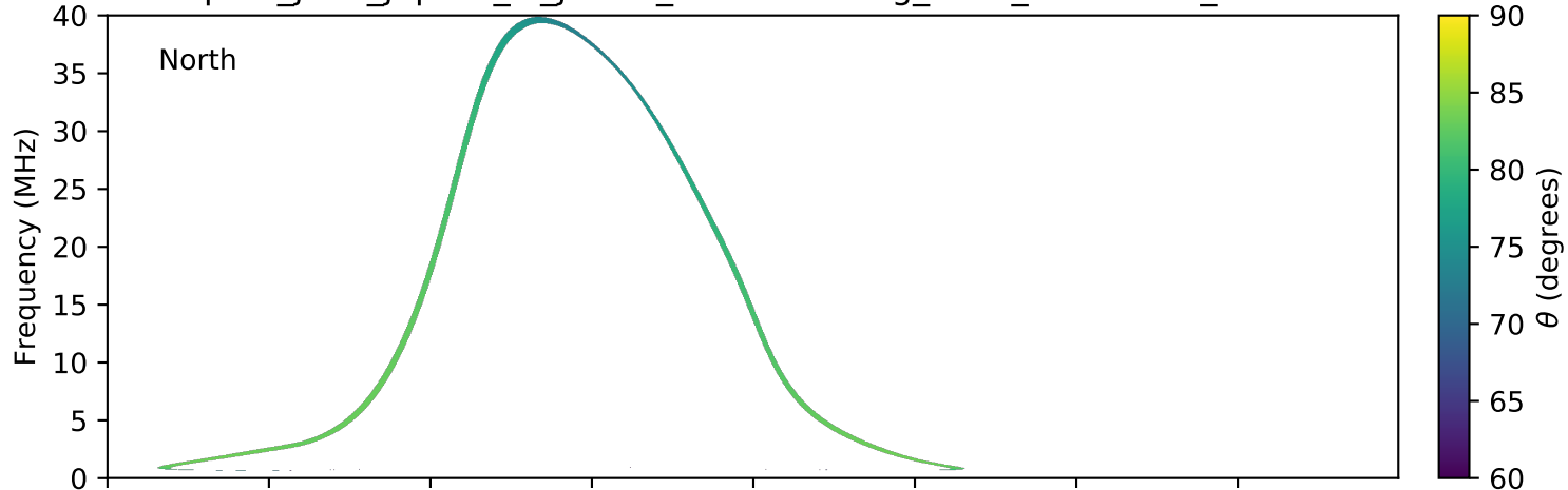
expres_juno_jupiter_io_jrm09_lossc-wid1deg_3kev_20180915_v01.cdf
