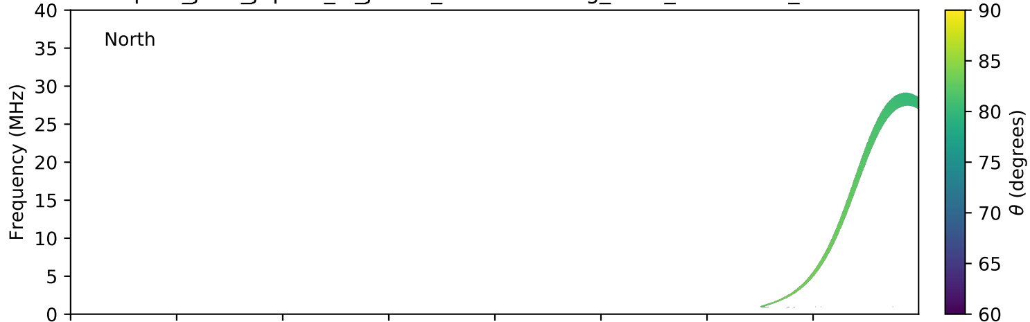
expres_juno_jupiter_io_jrm09_lossc-wid1deg_3kev_20180909_v01.cdf
