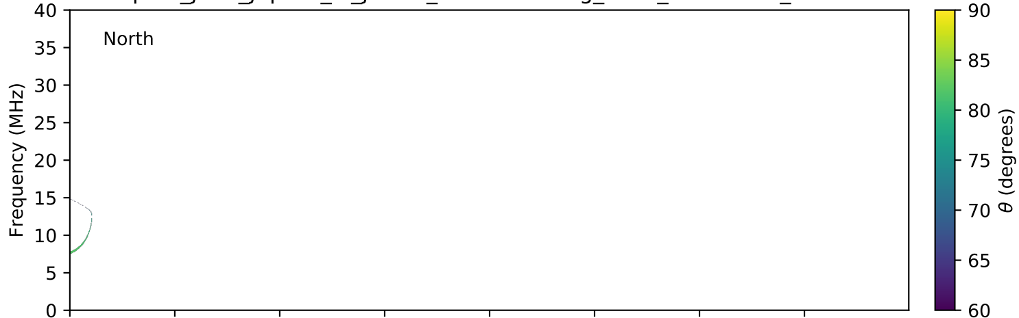
expres_juno_jupiter_io_jrm09_lossc-wid1deg_3kev_20180907_v01.cdf
