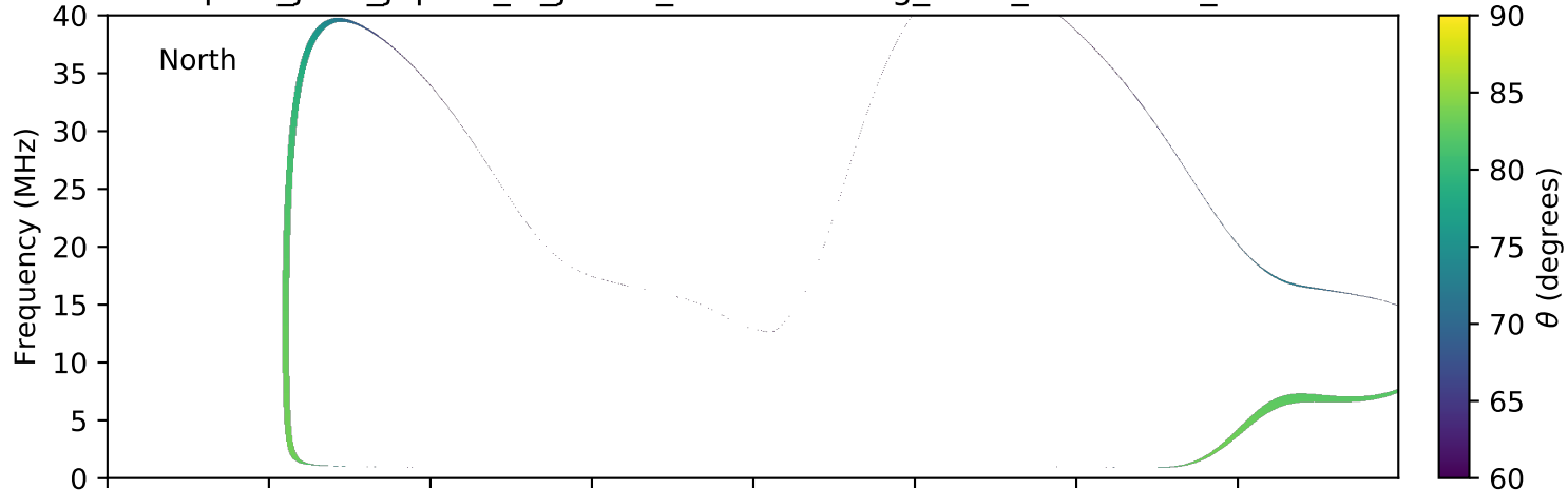
expres_juno_jupiter_io_jrm09_lossc-wid1deg_3kev_20180906_v01.cdf
